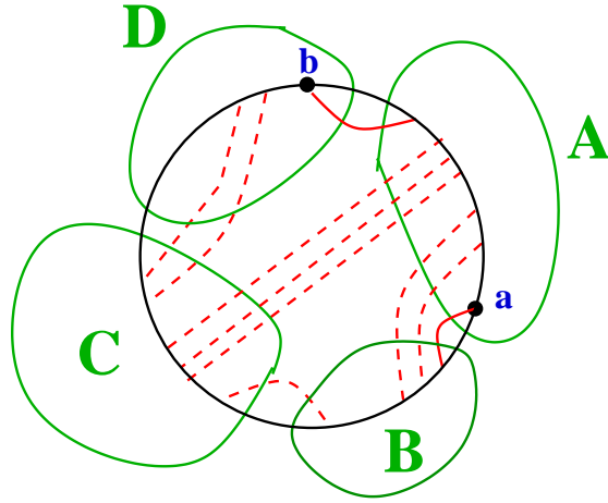
FIGURE 5. A reduced partition
