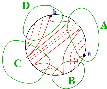
FIGURE 7. Reduced permutation with two simply twisted cycles
