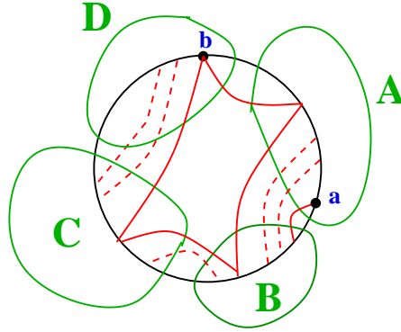
FIGURE 6. Reduced permutation with one doubly twisted cycle
