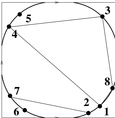
FIGURE 3. A representation of a genus 1 permutation on the torus
