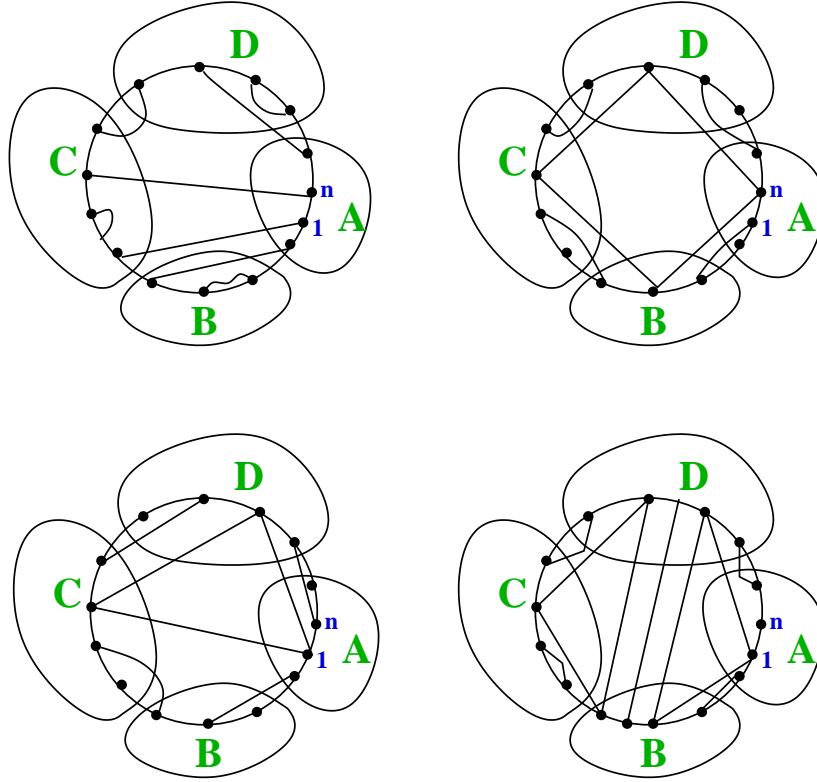
FIGURE 4. The four types of genus 1 permutations
