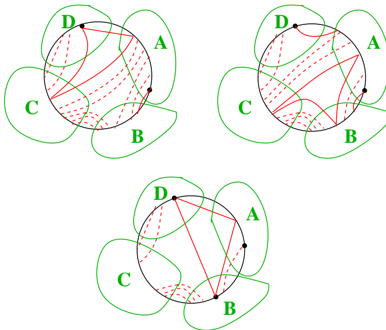
FIGURE 8. Three reduced permutations with one simply twisted cycle
