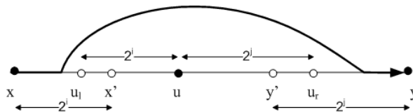
Figure 1: One-failure case, where the thick line denotes a detour of the third type.
